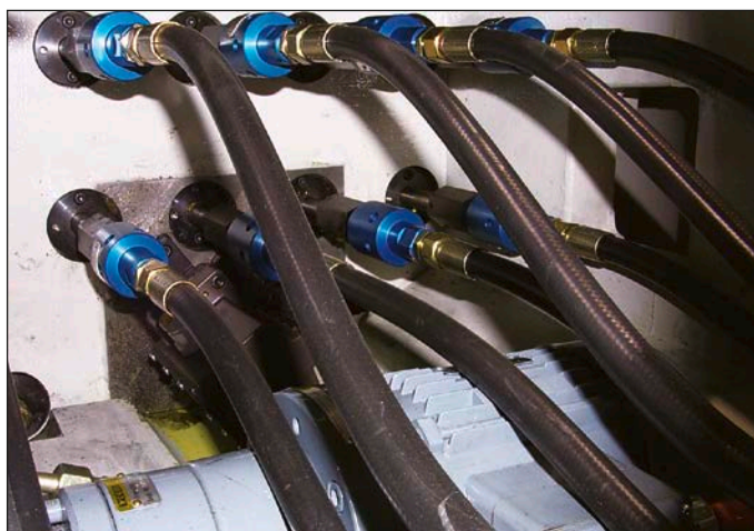
Deublin 1116 Bearing-Supported Unions on Automotive Transfer Line.
