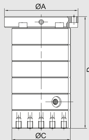
Rotor-mounted Axial Connection Connection 2
